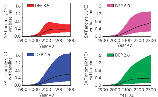
Figure 1 | Global average surface air temperature anomaly with respect to baseline runs with no carbon sequestered in permafrost soil layers.
